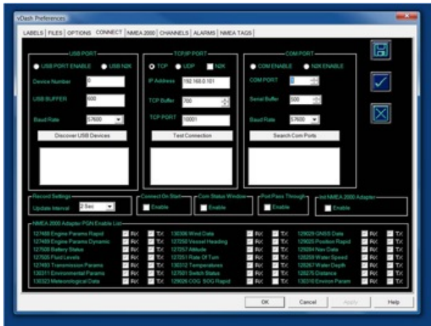
vDash Connect Screen with enabled TCP connection to SeaSmart.Net adapter using IP address 192.168.0.101 Port 10001
